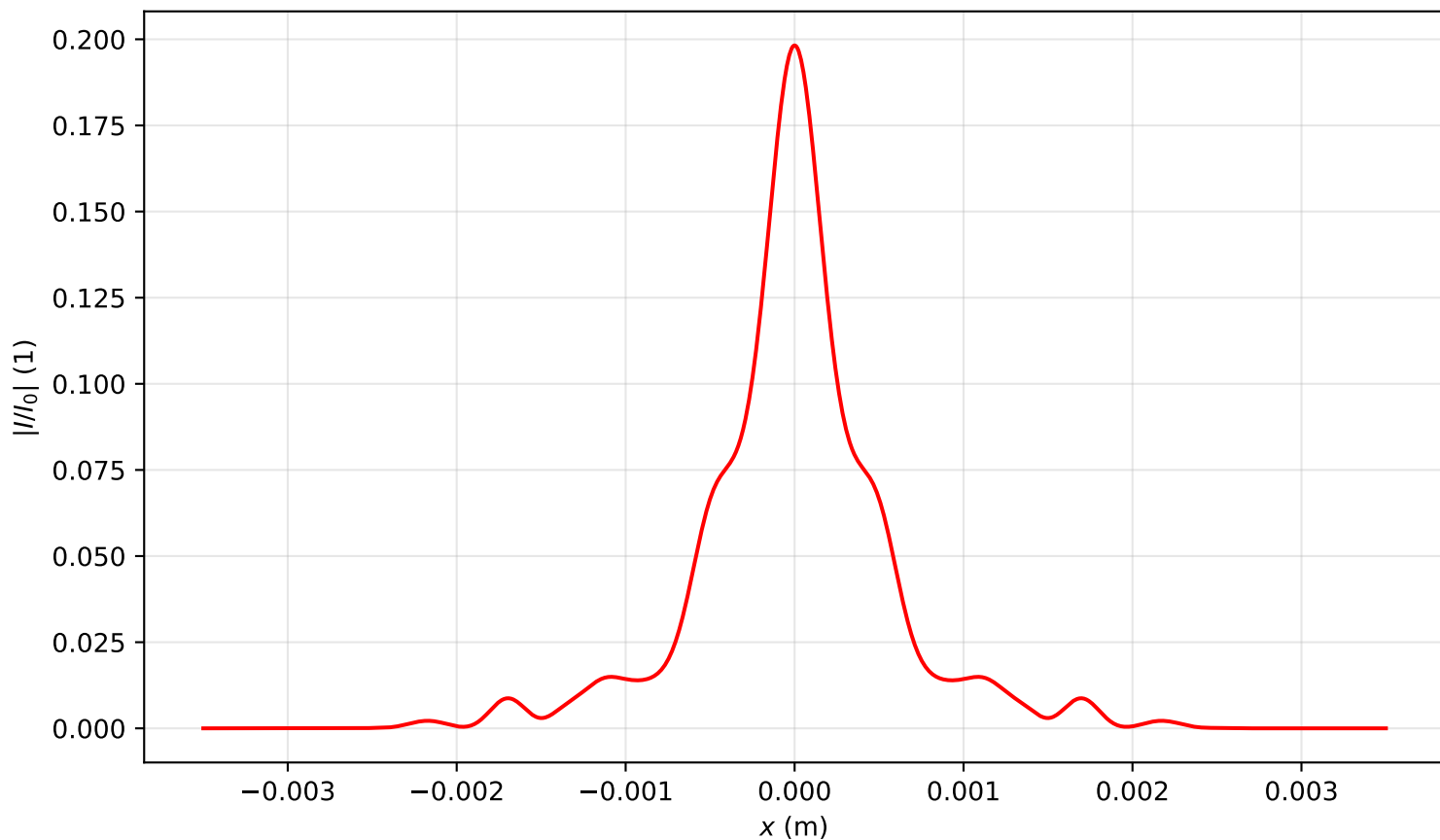
Intensity profile I(x, y = 0, z = 3.821)/I_0 , \text{Pin}=5.0\text{Pcr} , artificial time
